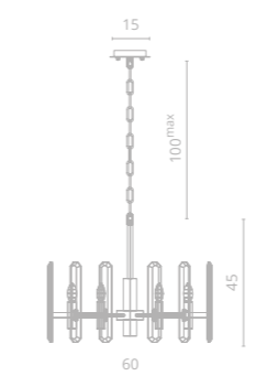
5 7136/18 LM-6 ∅60 | 145 | 100 max 6x60W E14
