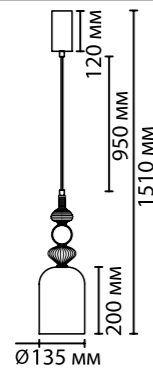
5045/12LA, 5046/12LA 1 x LED x 12W, 1400 lm крепеж: планка
