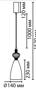
5045/12LC, 5046/12LC 1 x LED x 12W, 1400 lm крепеж: планка
