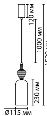
5045/12LB, 5046/12LB 1 x LED x 12W, 1400 lm крепеж: планка
