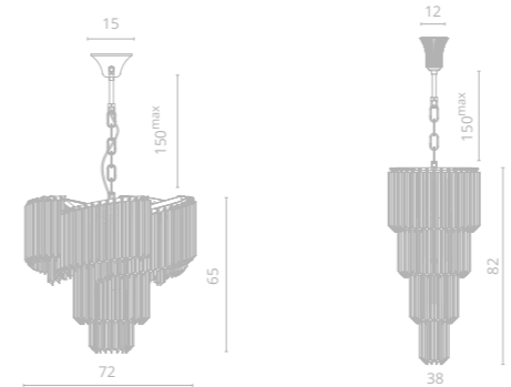
3 1681/01 LM-9 ∅72 | 165 | 150 max 9x60W E14 4 1681/01 SP-9 ∅38 | 182 | 150 max 9x60W E14
