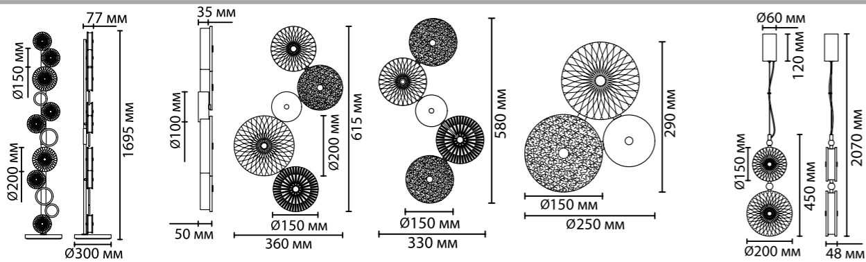
5412/13LA, 5412/13LB, 5412/13LC, 5412/13LD 1 × LED × 13W, 700 lm крепеж: планка
